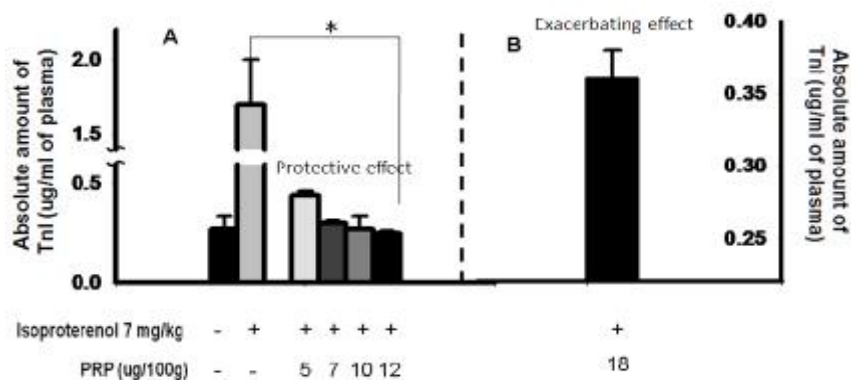
Fig.2. Cardio protective/deleterious effect of PRP, reflected by decrease of cTnI leakage into blood stream in the model Isoproterenol-induced cardiac impairment. A. In a dose dependant manner PRP I/P, which was administrated 2 hours before injection of Iso, decreased the amount of cTnI in blood stream. B. Increased dosage of PRP had a reversed, deleterious effect and increased the amount of cTnI in blood. Unless specified otherwise, the data are shown as a mean S.E.M. n = 3 rats per group; p < 0.05 between control and groups of the animals received PRP.
